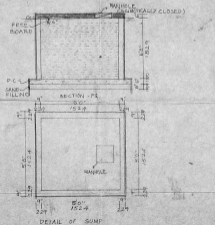
DETAIL OF SUMP
