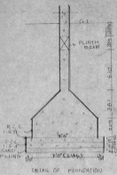
DETAIL OF FOUNDATION
